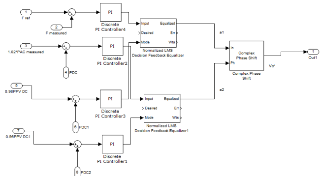
Fig. 8. Modification of PV inverter frequency control loop.
