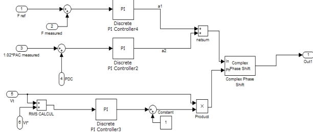
Fig. 9. Integrated Solar PV MPPT and PQ control diagram.
