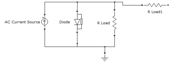
Fig. One Diode Equivalent circuit of Solar PV
