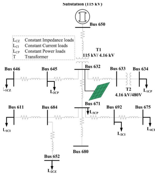
Fig. 4. IEEE-13 bus distribution feeder.
