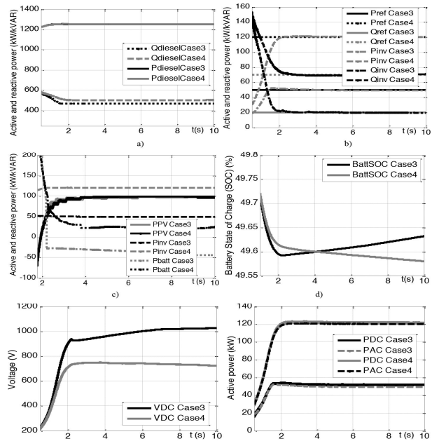
Fig. 15. Results of coordinated P-Q control with solar PV including MPPT control and battery control.
