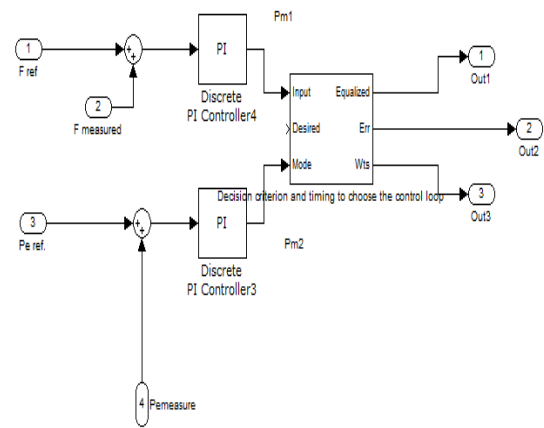
Fig. 7. Diesel generator control transition.
