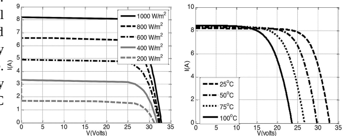
Fig. 2. The I - V characteristics of Kyocera KC200GT from simulation with (a) varying irradiance at a cell temperature of 25°C and; (b) varying cell temperature at 1000W/m 2
