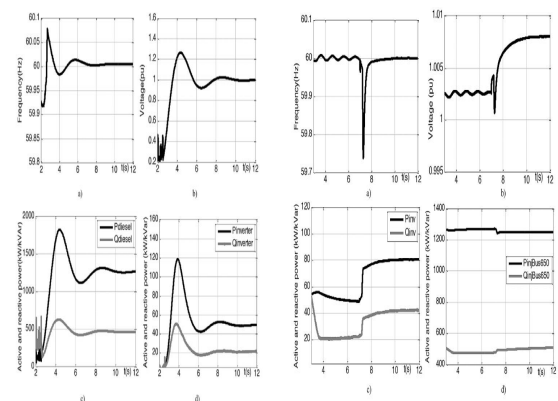
Fig. 11. Results for V-f control of microgrid with diesel generator & Fig. 12. Results of V-f control showing grid to microgrid transition.
