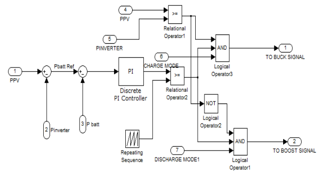
Fig. 6. Battery power control diagram.
