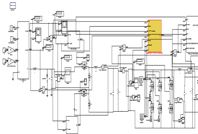
Fig. 10. Matlab Simulink model of coordinated V-f control with solar PV including MPPT control and battery control of
