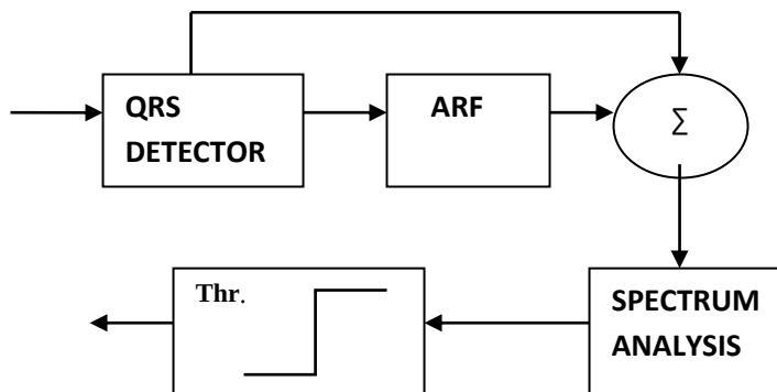
Fig. 2: The schematic of the adaptive recurrent filter ARF
