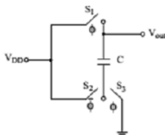
Fig. 1 Voltage Doublers using charge pump
