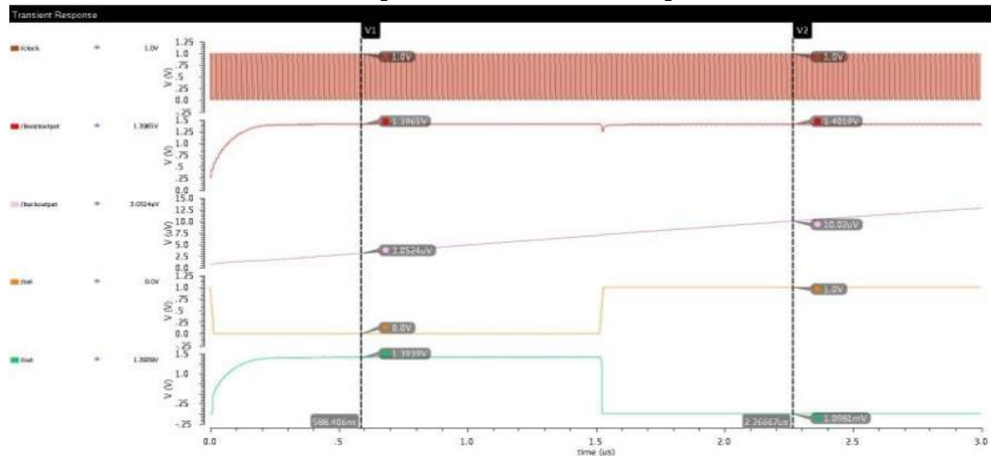
Figure 6 Transient Analysis of Buck-Boost Converter with multiplexer
