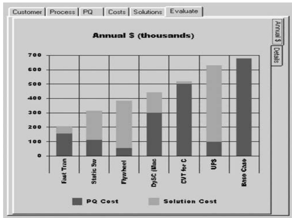
Figure 2. Comparing solution alternatives with the base case using total annual costs
