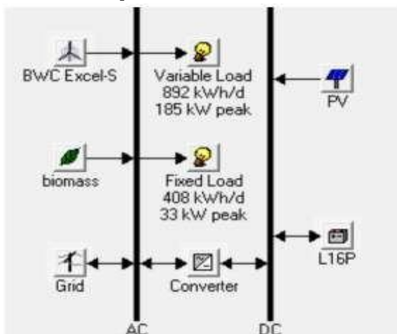
Fig 7.5 distribution set up
