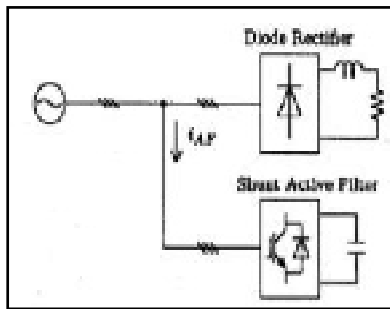
Fig 4.2: Shunt active filter used alone
