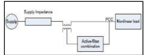
Fig 4.6: Combination of shunt & series active filters
