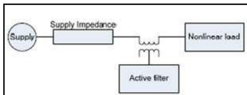
Fig 4.4: Series active filter configuration
