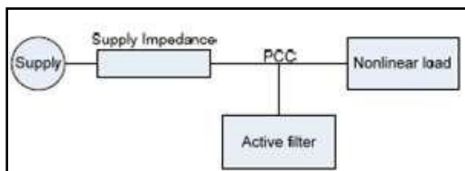
Fig 4.3: Shunt active filter network configuration
