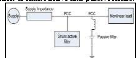
Fig 4.8: Shunt active & shunt passive filter combination ➤ Active filter in series with shunt passive filters:
