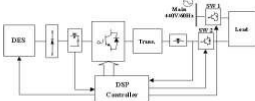
Fig 2.5: Block diagram of power converters connected in parallel
