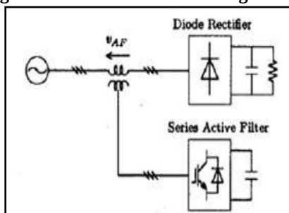
Fig 4.5: series active filter used alone
