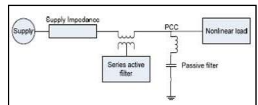
Fig 4.7: Series active & shunt filter combination
