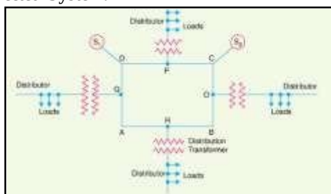
Fig 5.3: Inter-connected System
