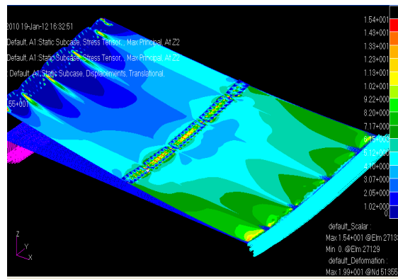
Figure 3(b) maximum stress concentration at bottom skin splice joint.
