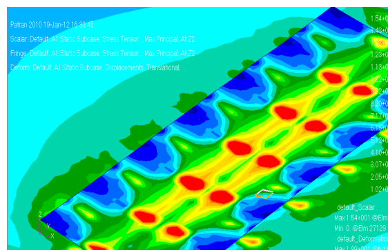
Figure 3(c) maximum stress at rivet holes of the splice plate
