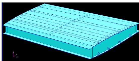
Figure 1(a): CAD model of Wing box (CATIA V5R19)
