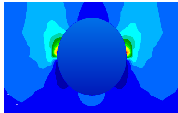
Figure 3(d) maximum stress near splice joint rivet hole.
