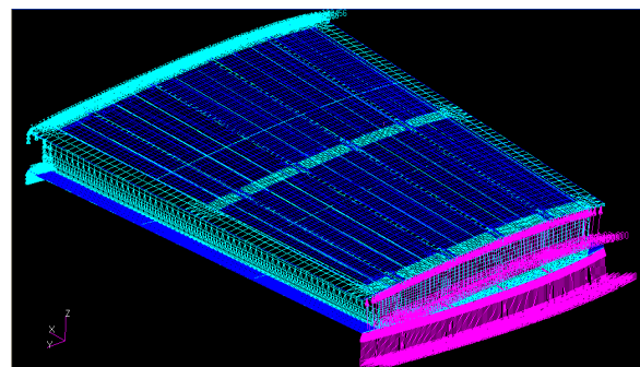
Figure 3(a) wing box loading conditions
