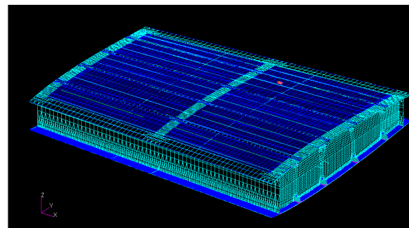
Figure 2(a) Meshed model of wing box
