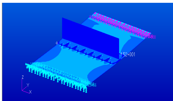
Figure 3(d) local analysis on splice joint
