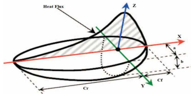
Fig 1. Double ellipsoidal heat source [8]
