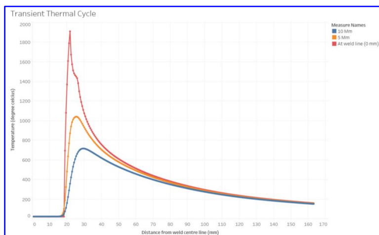
Fig. 5. Transient temperature history profile
