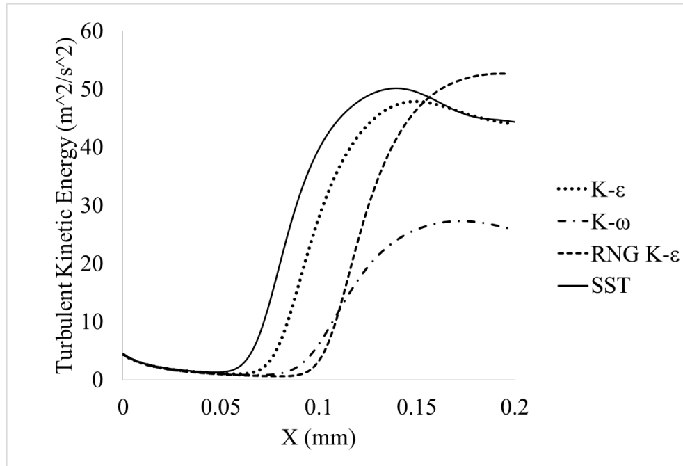
Fig 3 Centerline turbulent kinetic energy distribution
