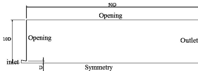
Fig 1 Domain dimensions and boundary conditions
