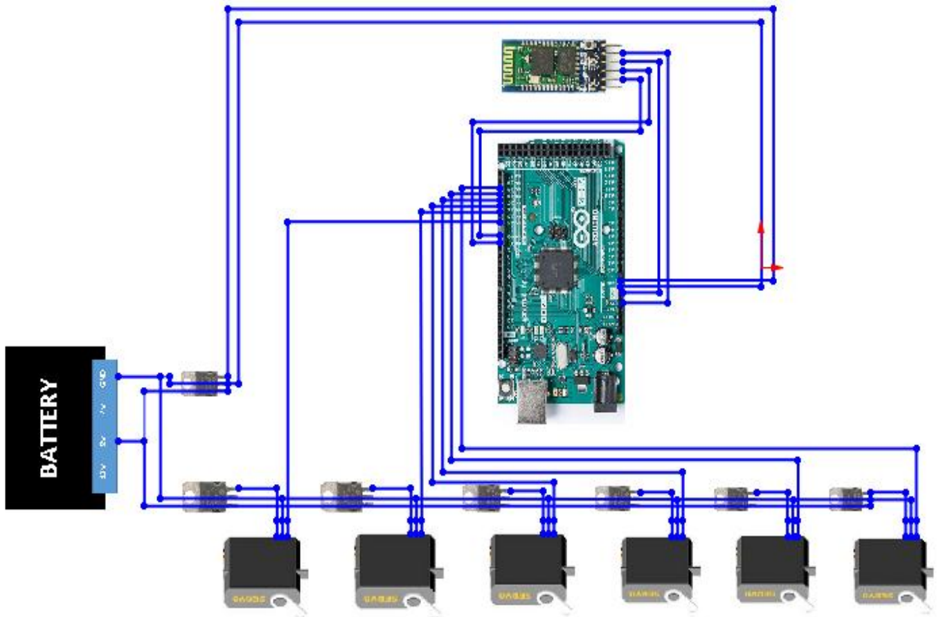
Figure 17: Arduino Interfacing with Bluetooth Module and Servo Motors
