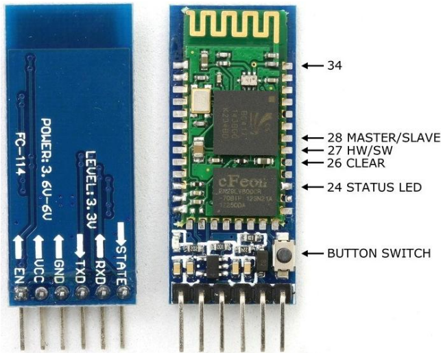
Figure1: Bluetooth Module HC-05
