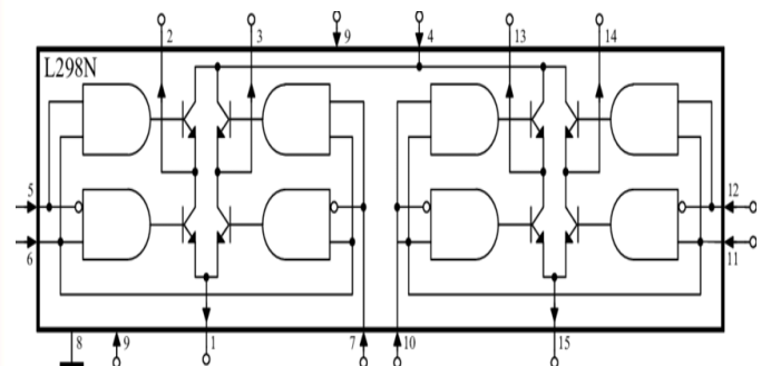
Figure4: Dual H-Bridge Circuit
