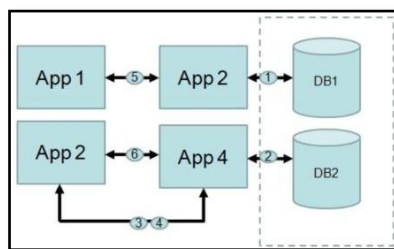
Figure 1: Migration of Legacy system
