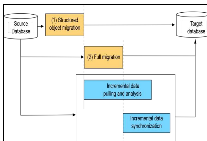
Figure 2: Example of data migration through reverse engineering
