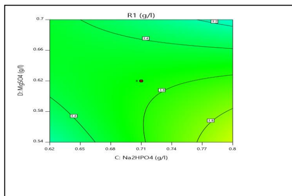
Fig. 1 Contour plots showing the combined effect of the medium variables (glucose , ammonium sulfate ,magnesium sulfate and sodium hydrogen phosphate) on EPS production by AB4 Pseudomonas aeruginosa
