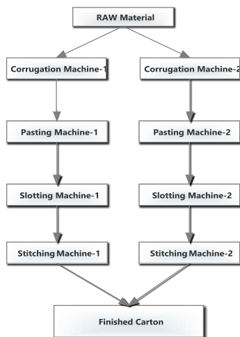
Figure 2. Process Flow of corrugated box manufacturing plant
