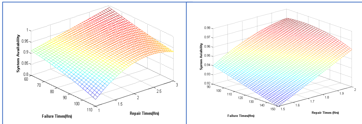
Figure 6. Effect of Failure (Repair) times of the Machine on system availability of the Slotted Machine on system availability
