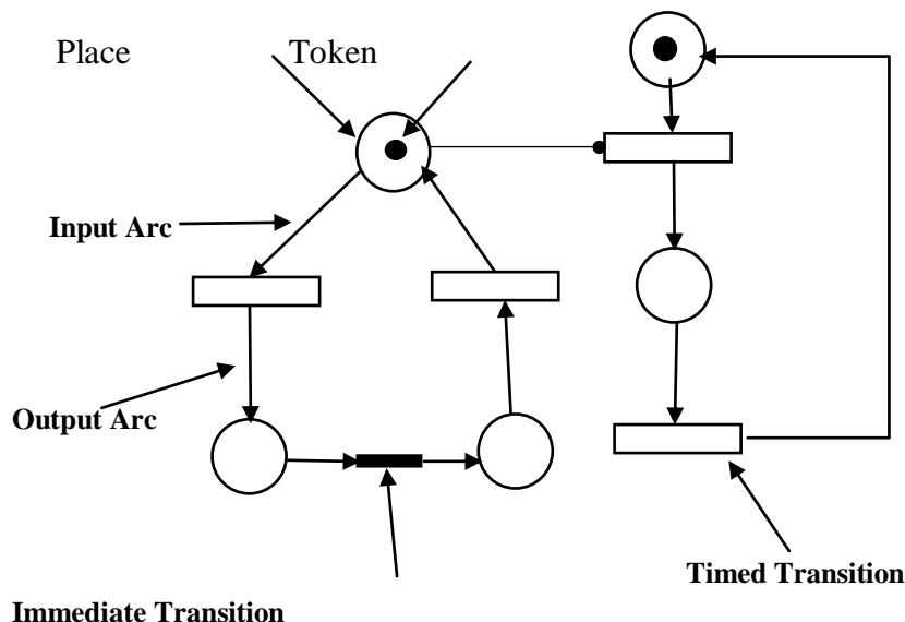
Figure 1. Petri Net
