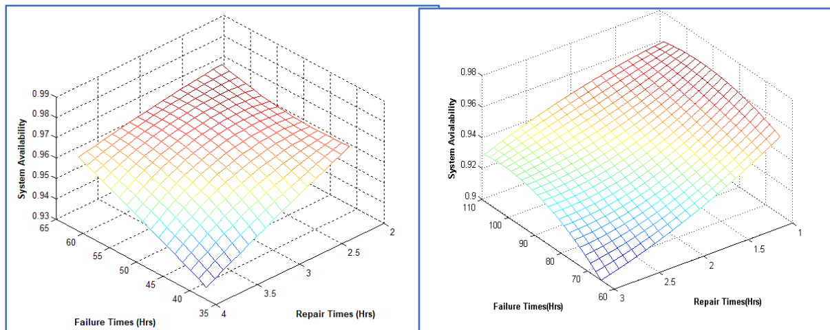
Figure 4. Effect of Failure (Repair) times of the Figure 5. Effect of Failure (Repair) times Corrugation Machine on system availabilityof the Pasting Machine on system availability
