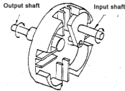
Fig. 15: Internal Geneva Mechanism
