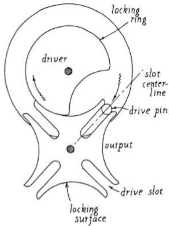
Fig. 14: External Geneva Mechanism
