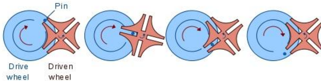
Fig. 1 Geneva Wheel Rotation
