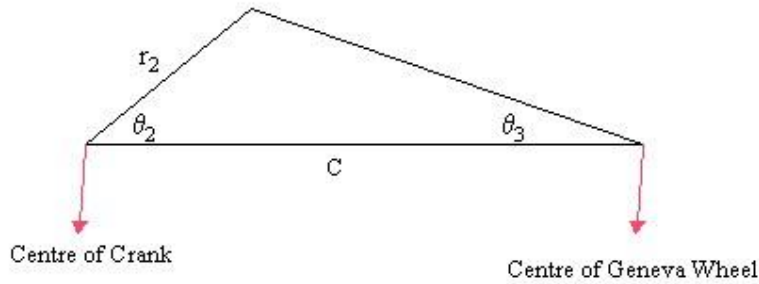
Fig. 12: Position of Geneva Wheel
