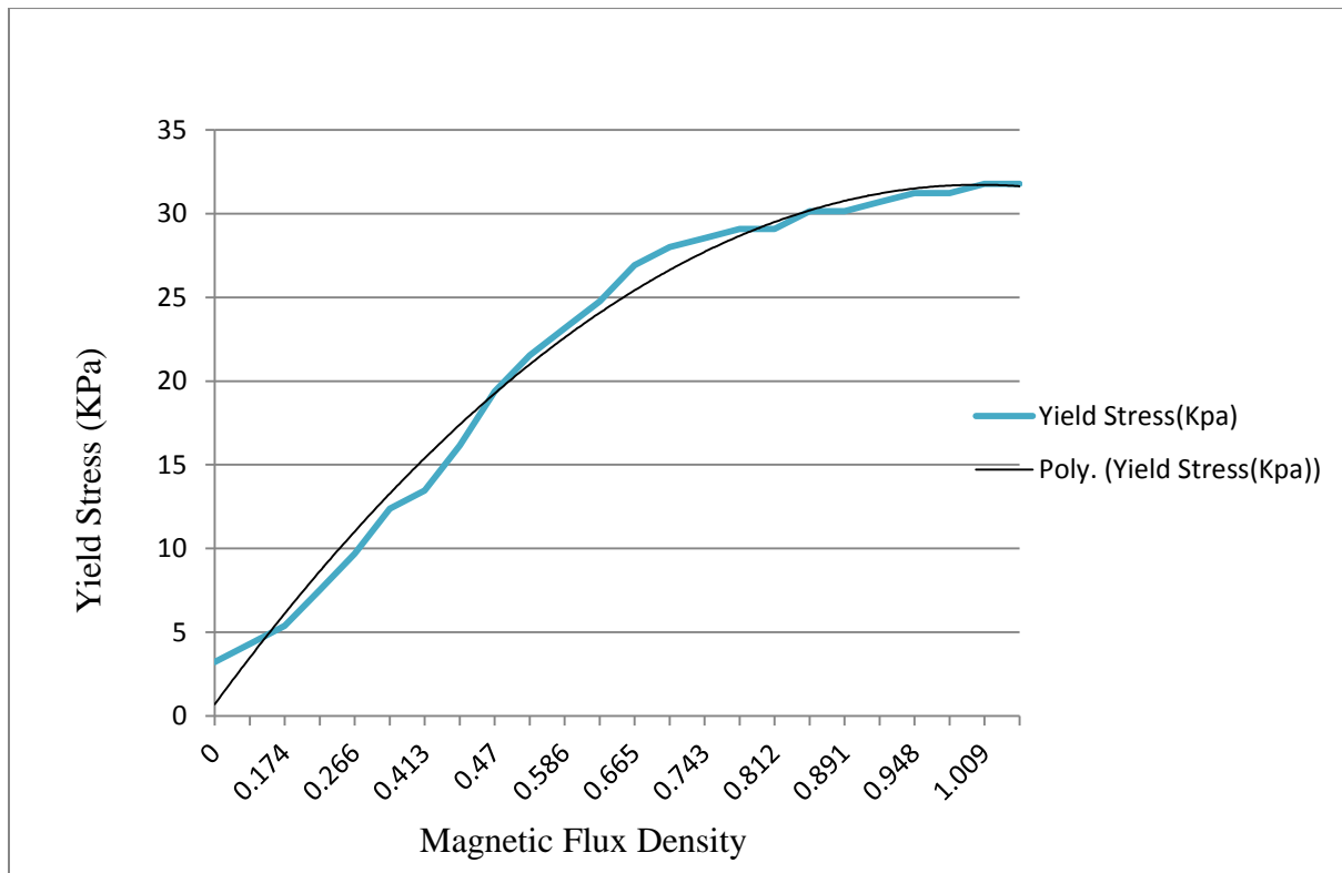
Fig. 1: Plot of experimental values between Yield Stress and Magnetic Flux Density
