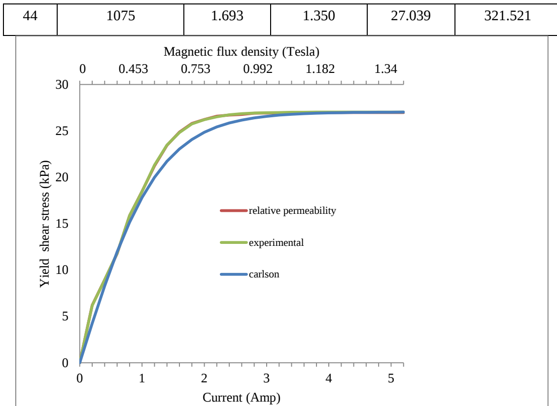
Fig. 1 Variation of yield shear stress with magnetic flux density for sample 1 by different approaches
